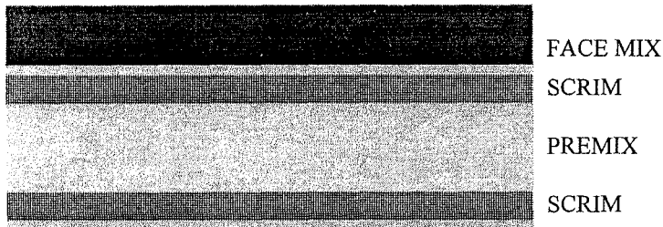
Figure 2-Test Panel Configuration
